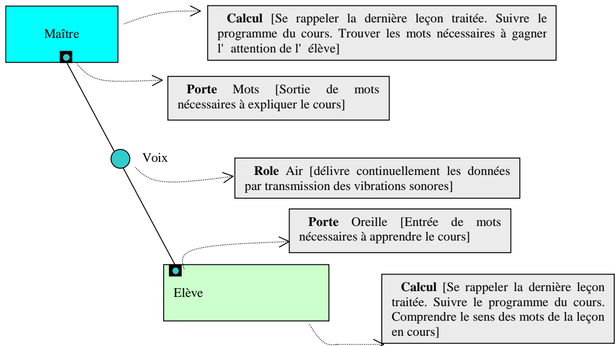
Figure 2.2 : Architecture Cours
