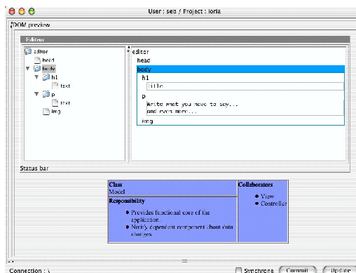
Figure 3. SAMS-XML environment
