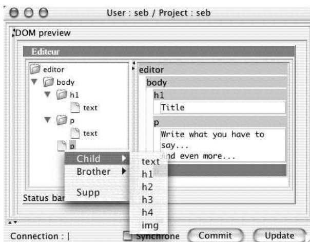
Figure 2. SAMS-XML editor
