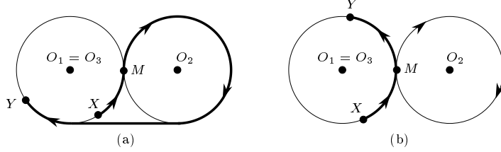
FIG. 5.6. When O_1 = O_3 : (a) \Pi(M) is of type C_1^+ C_2^- S C_3^- ; (b) \Pi(M) of type C_1^+ C_2^- S C_3^+ degenerates to a single C -segment, for any M \in \mathcal{C}_1 .
