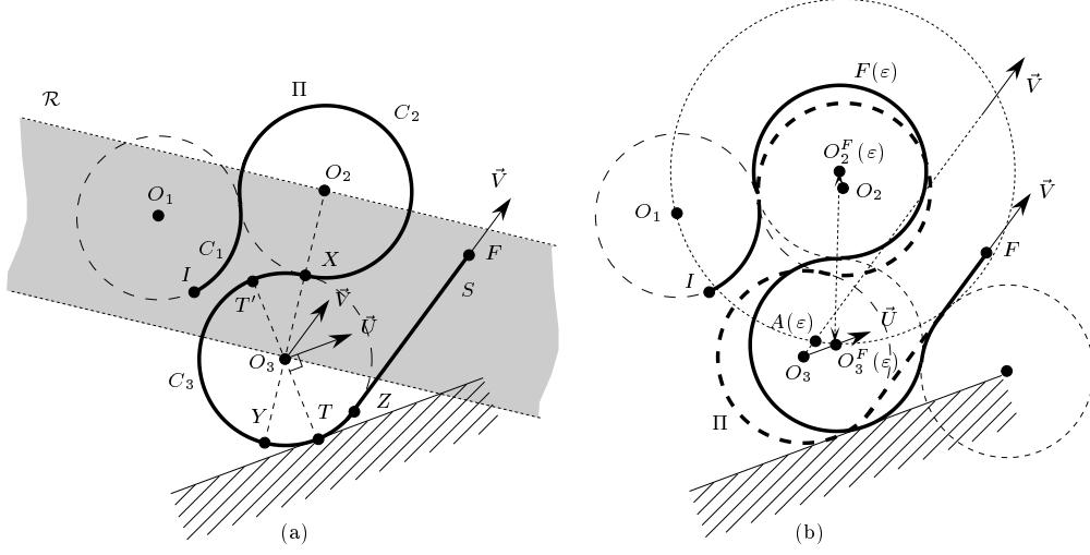
FIG. 3.5. (a): Path \Pi . (b): A shorter path F(\varepsilon) .
