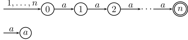
Fig. 9. Deterministic STA for the language T_n of Proposition 27.
