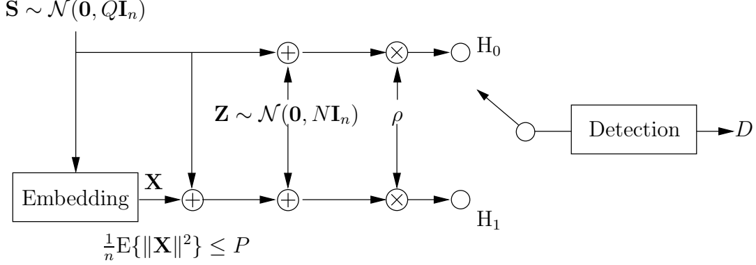
Figure 2. Equivalent framework
