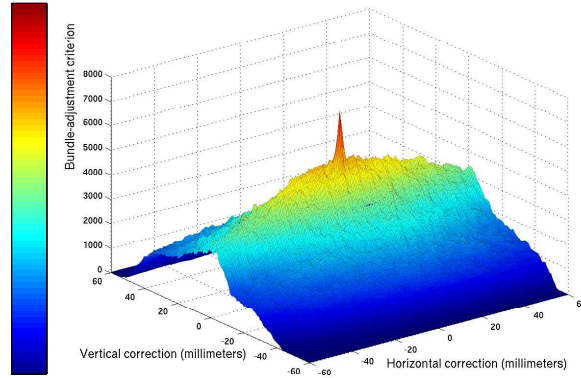
Figure 14: Global matching criterion value with respect to vertical and horizontal translations of one of the reference images. A maximum clearly occurs at the correct image translation.
