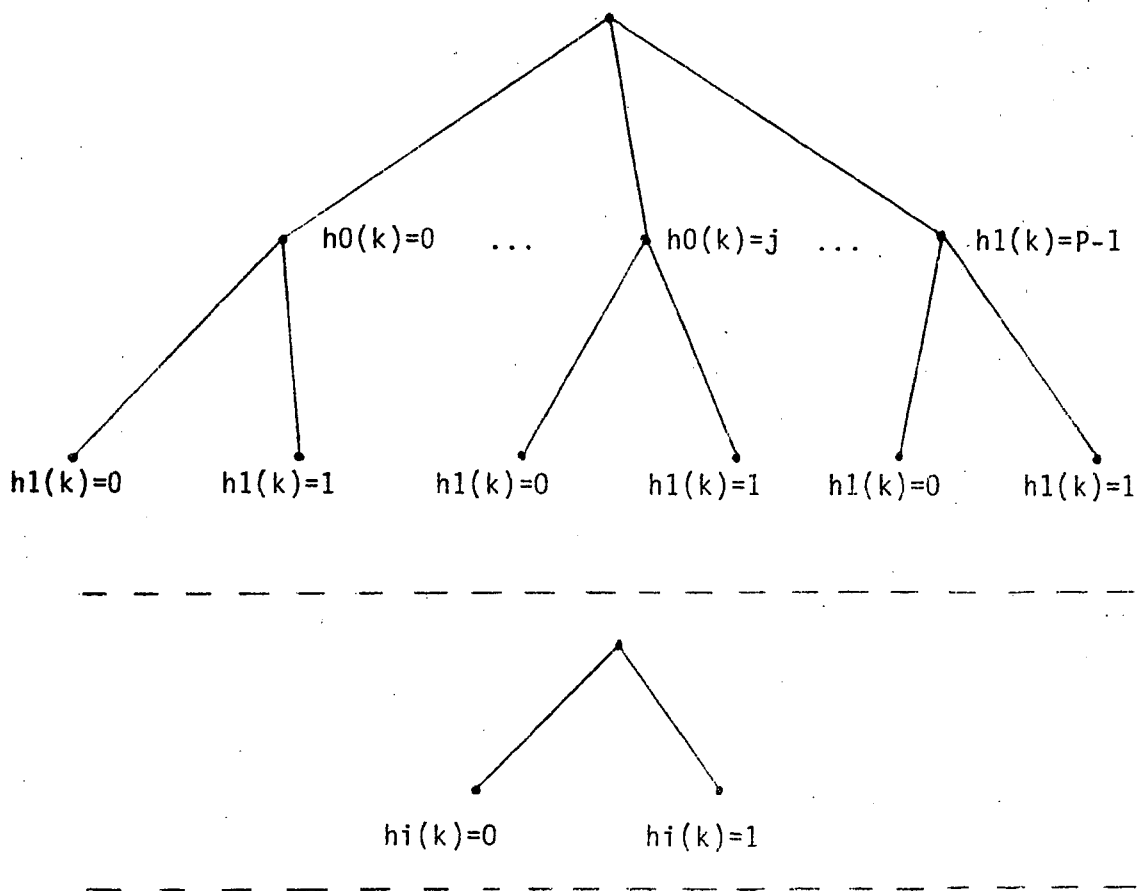
Figure 6. : PT for extendible hashing
