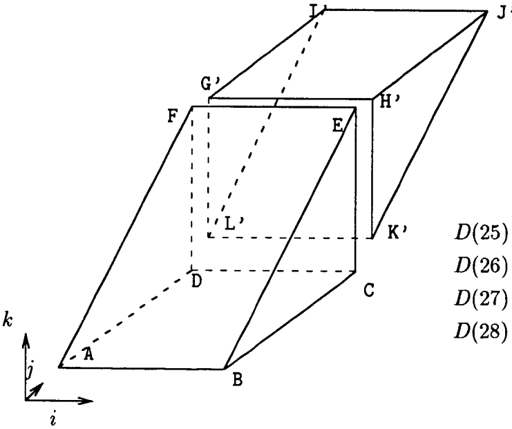
Figure 8: Translation of the subdomain j < k
