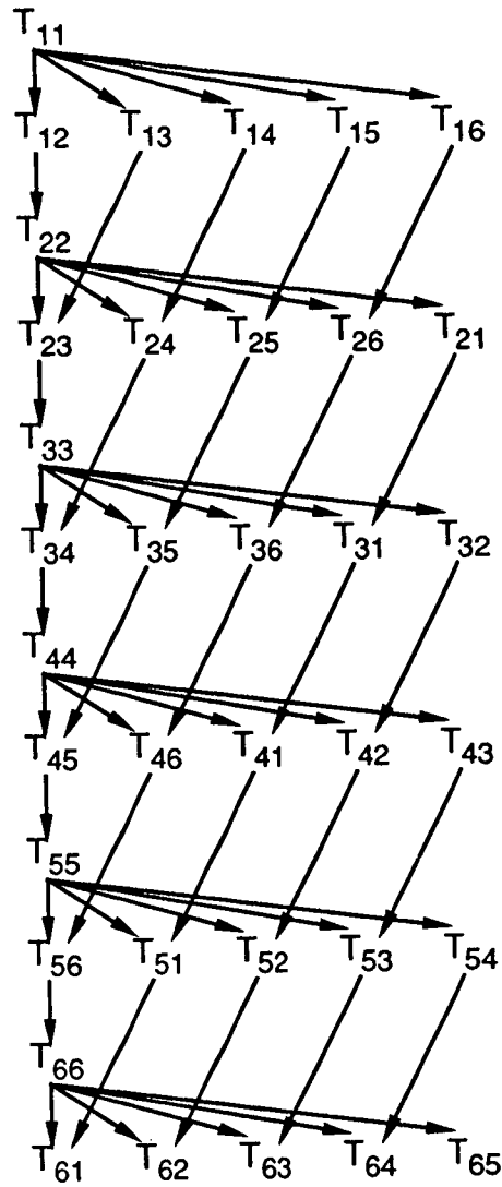
Figure 1: Task graph for the APP ( n = 6 )
