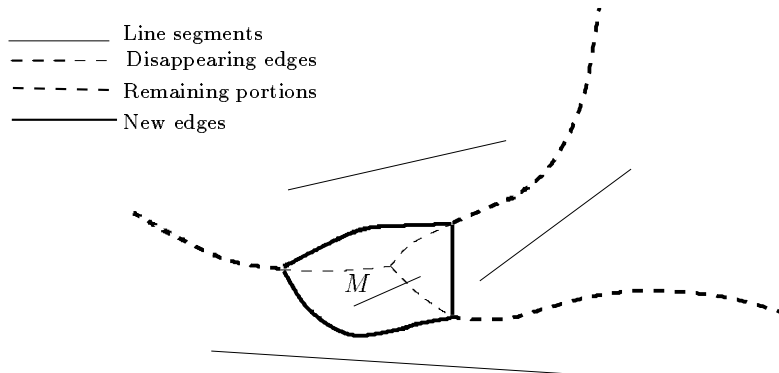
Figure 5: Insertion of a new segment in a Voronoi diagram.
