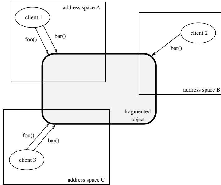
Figure 2.1: A fragmented object as seen from clients
