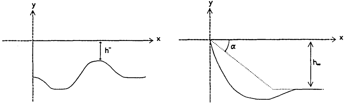
Figure 7: (i) h^- > 0
