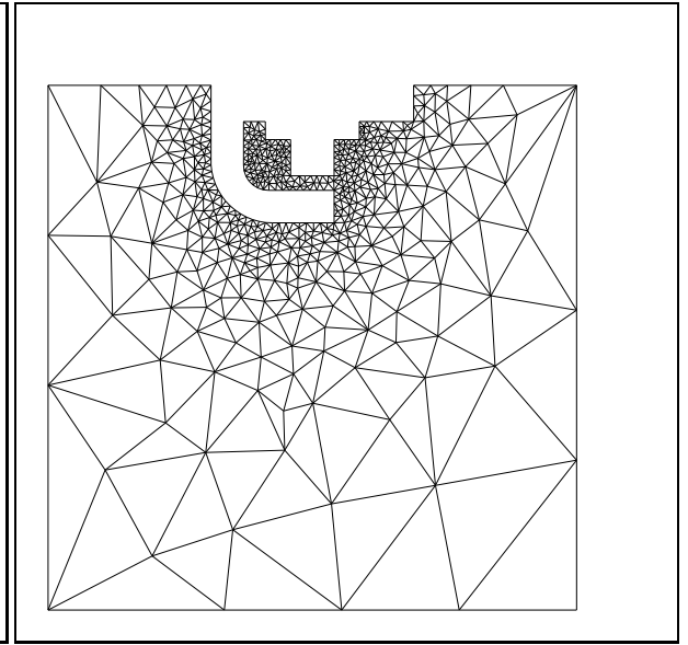
Figure 3.b : after one coarsening
