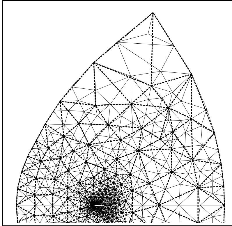
Figure 1. Partial view of the initial and first coarsened meshes
