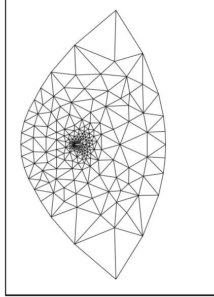
Figure 2.b : after one coarsening
