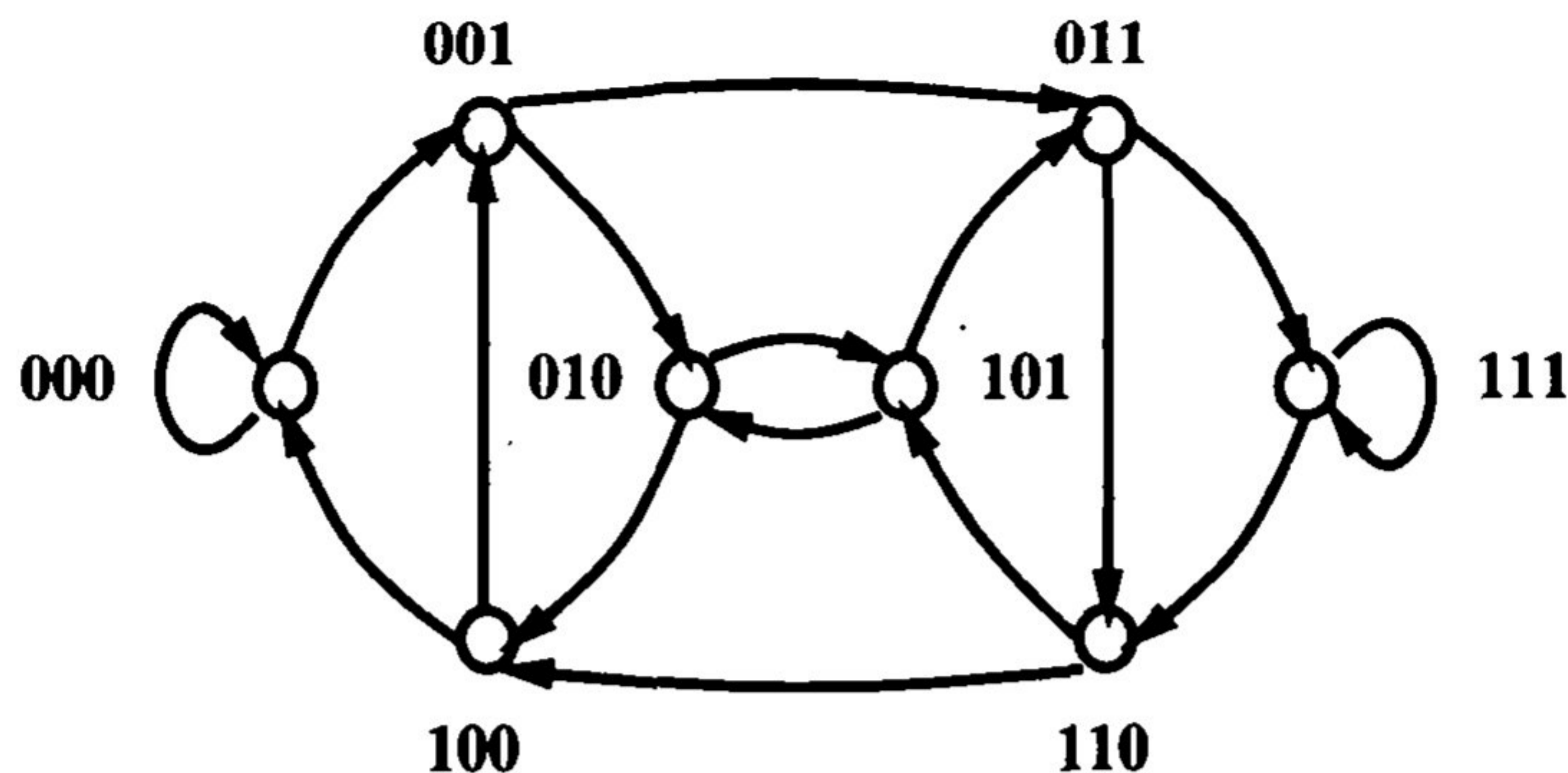
Figure 1: Example of a de Bruijn digraph B(2, 3) .
