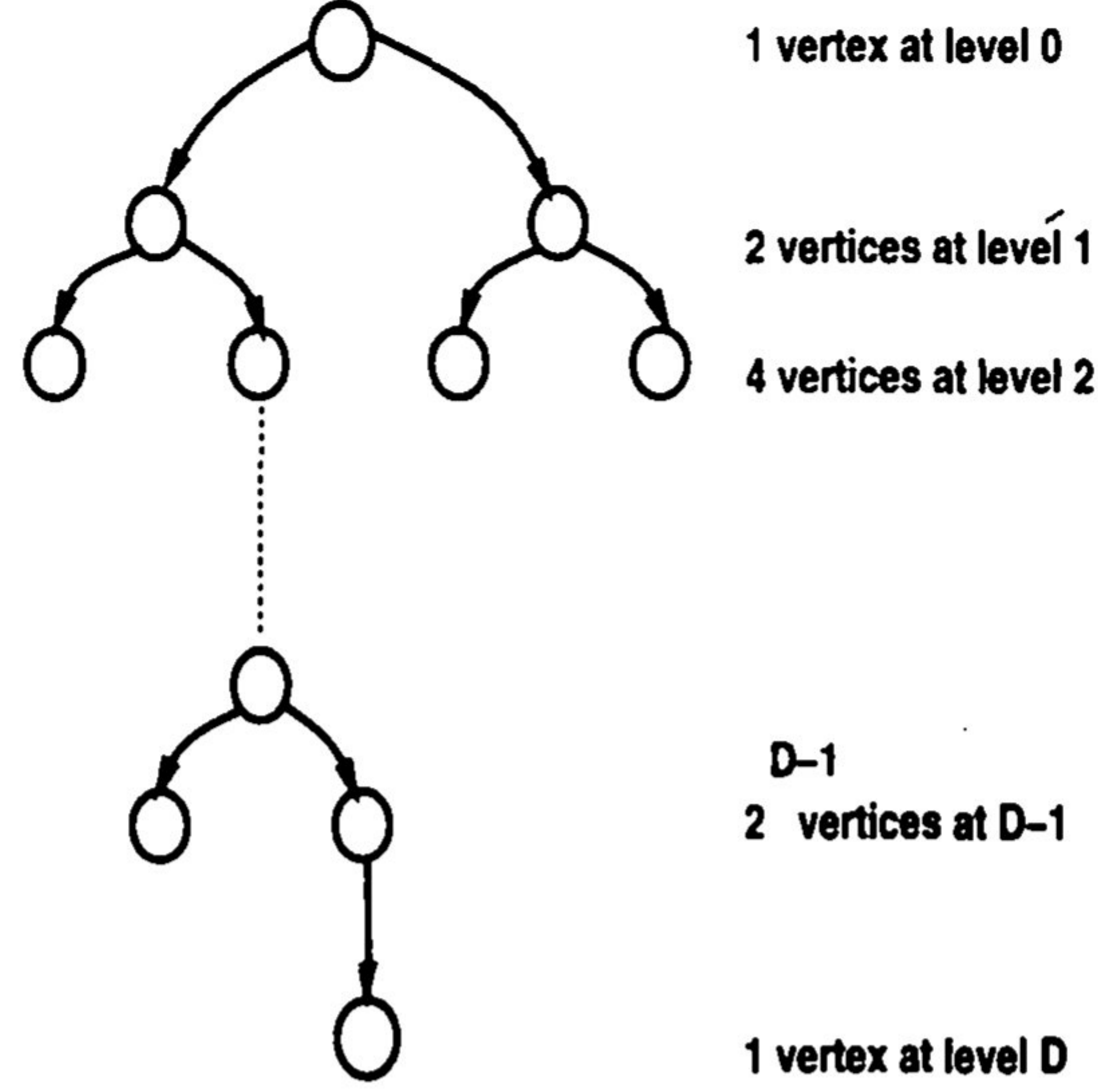
Figure 2: Shortest path tree with the minimal weight
