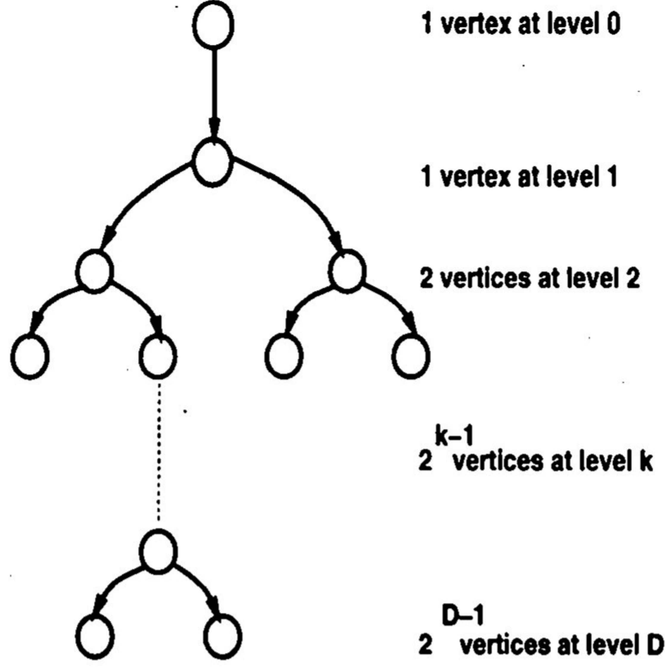
Figure 3: Shortest path tree with the maximal weight
