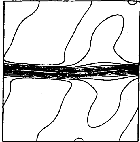
Figure 4: Contour-values of the spectral method, 61 \times 81 collocation points, Ma_c = 0.8 , Re = 400 , Pr = 0.7 , L_x = 20\delta_i , t = 20
