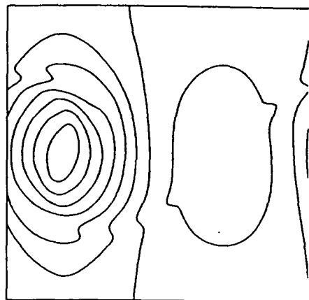
Figure 2: Contour-values of the 2nd order FV-solver, random perturbation, 101*101 grid-points, Ma_c = 0.3 , Re = 1000 , Pr = 0.7 , L_x = 15.06 \cdot \delta_i , t = 95
