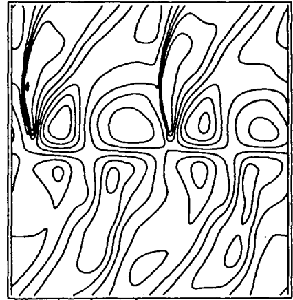
Figure 21: Contour-lines of u_c : 101 points in x (left), 401 points in x (right), t=120
