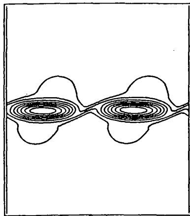
Figure 16: Contour-lines of entropy with 101 points (left) and 401 points (right), Ma_c = 0.8 , Re = 1000 , Pr = 0.7 , L_x = 22.52 \cdot \delta_i , t = 60
