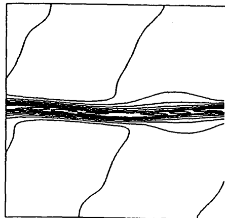
Figure 5: Contour-values of the 2nd order FV-solver, 101 \times 101 grid-points, Ma_c = 0.8 , Re = 400 , Pr = 0.7 , L_x = 20\delta_i , t = 20
