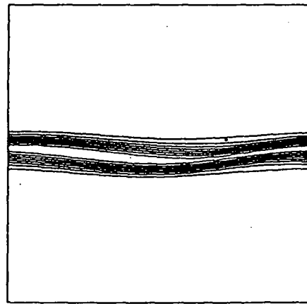
Figure 5: Contour-values of the 2nd order FV-solver, 101 \times 101 grid-points, Ma_c = 0.8 , Re = 400 , Pr = 0.7 , L_x = 20\delta_i , t = 20
