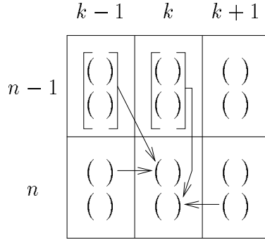
Figure 3: Computation of cell (n, k) .
