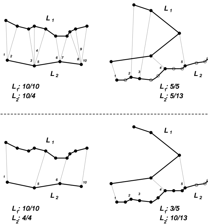
Figure 4: The topological constraints help to remove inconsistent couples of linked points: left, some points have too many correspondents, right, a part of L_1 have a erroneous correspondent on L_2 .
