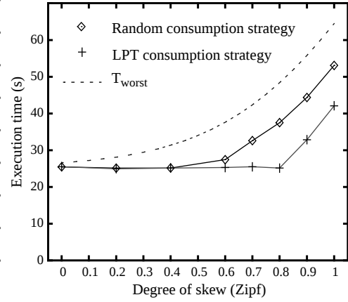
Figure 13: Ideal Join execution time
