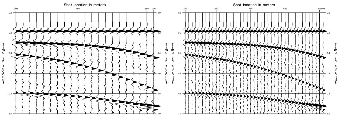
Figure 11: Synclay zero-offset gathers. Left: 21-shot set, right: 41-shot set.
