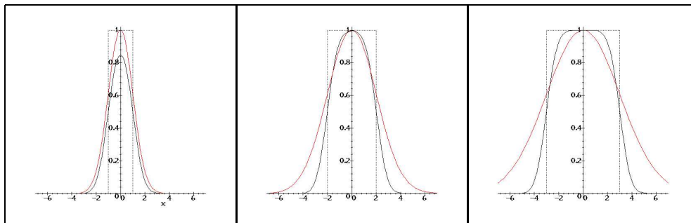
Figure 5: Illustration of the 1D bar-like convolved model. From left to right: models for a 1D vessel with radius 1,2 and 3. In red, a normalized Gaussian model. In black, convolution of a bar-like model with a Gaussian of standard deviation 0.7.
