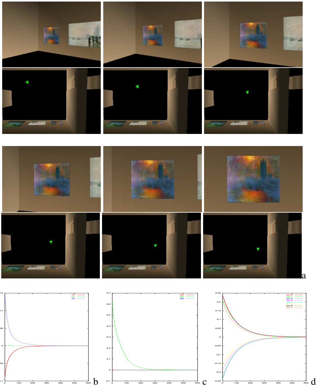
Figure 6: Positioning with respect to a painting (visual features are the four corners of the rectangle) (a) six camera and bird's eye views (b) camera translational velocities (c) camera rotational velocities (d) errors \mathbf{P} - \mathbf{P}_d in the image.
