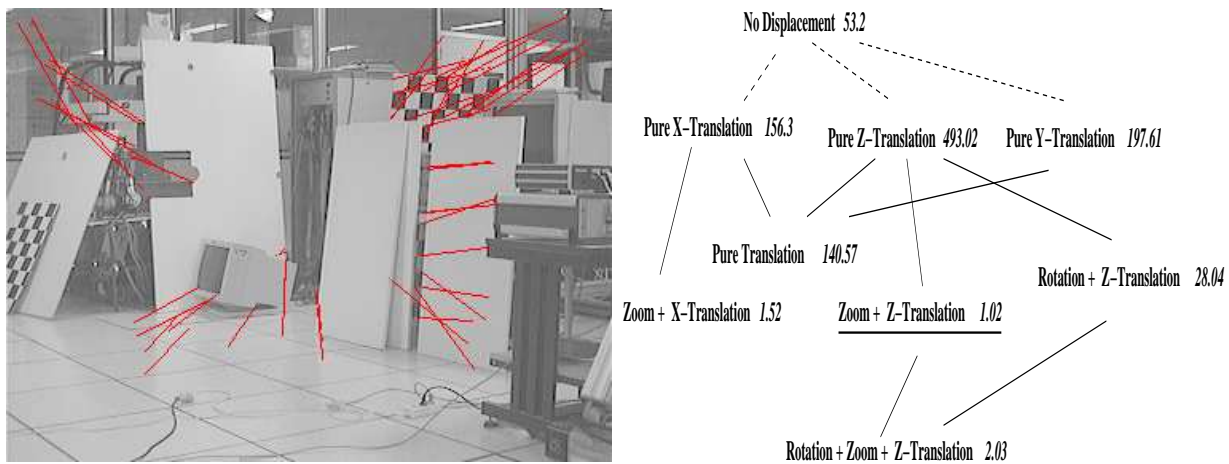
Figure 14: A partial view of the model hierarchy for a specific displacement estimation. See text for details. The displacement was a zoom of the camera.
