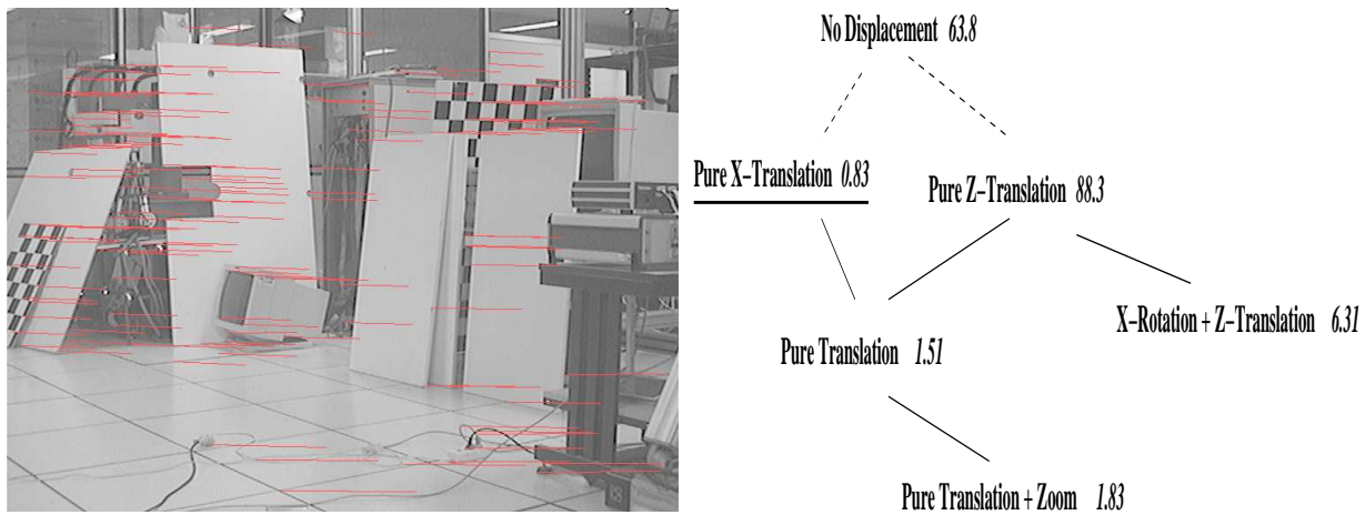
Figure 13: A partial view of the model hierarchy for a specific displacement estimation. See text for details. The displacement was a pure translation in the X-direction.
