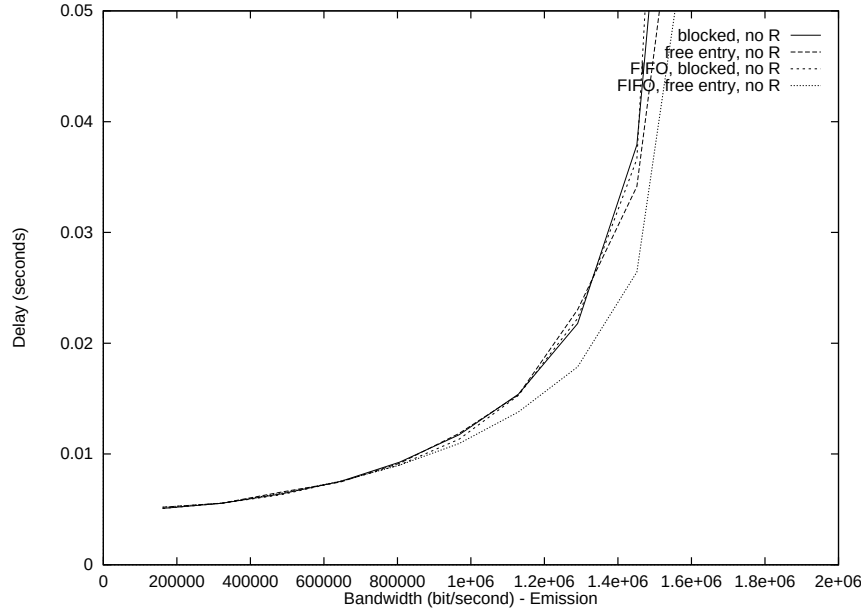
Figure 2: Average delay versus input load.
