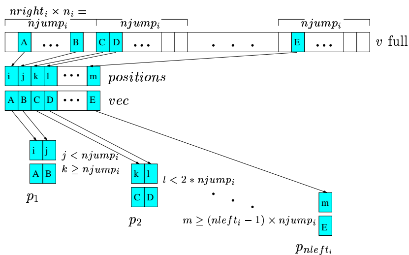
Figure 6: Separation of a reduced vector into l -slices, p_l
