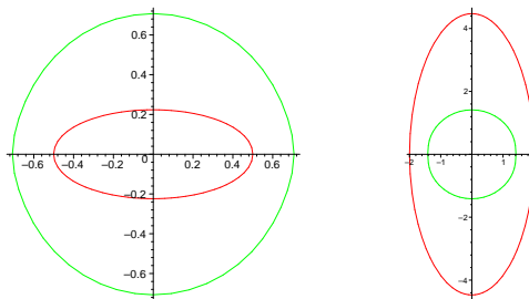
Figure 6: Slowness curves and Wave fronts for the orthotropic medium (I).
