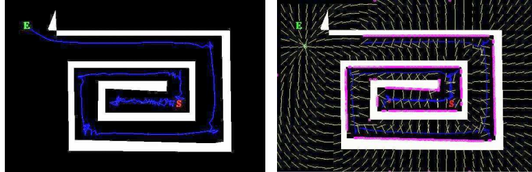
Figure 4: Showing the behavior of the mechanism in a “labyrinth” experiment. In the left view, the trajectory is starting at S and ending at E . At the beginning, attracted by the goal the trajectory starts in the wrong direction; then, because of obstacle repulsion, it finds its way out. At each change of direction, some trials are required to obtain a correct repulsion in order to be driven towards the goal. In the right view, “control” points onto the obstacle (in magenta ) and the potential field gradients (in yellow ) are drawn. The potential field has indeed no singularity except on the goal. We observe that a minimal number of points, i.e. the closest point to the obstacle, are used.
