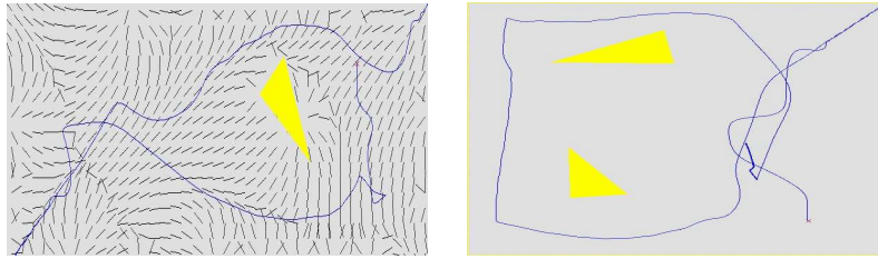
Figure 11: Showing how the same mechanism is used in the absence of any goal. As expected, a wandering behavior is generated. In the left view, the potential generated during the trajectory is shown, the geometry of the field is clearly induced by the geometry of the obstacles. In the right view, it is made visible that some parts of trajectory corresponds are straight and some are bended with several walk around the same position. These two qualitative effects are directly related to the evolution of the potential.
