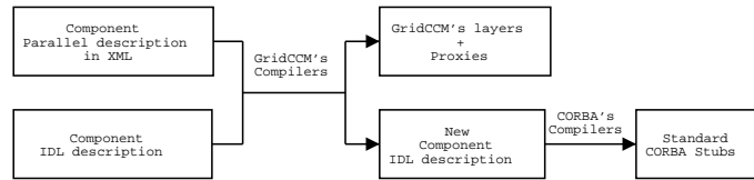
Figure 5: The different compilation phase to generate a parallel component
