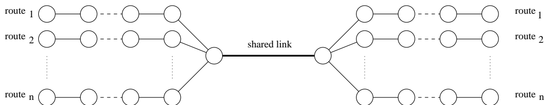
Figure 7: Dogbone topology
