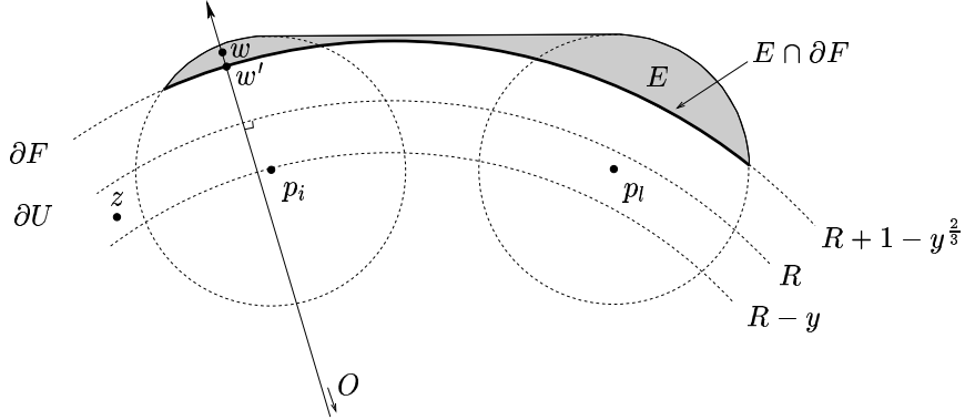
Figure 11. The part E of \mathcal{H}(p_i, p_l, 1) outside F .
