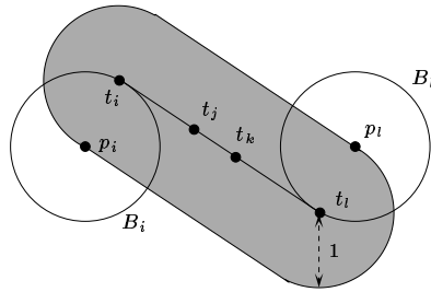
(b) \mathcal{H}(t_i, t_l, 1)
