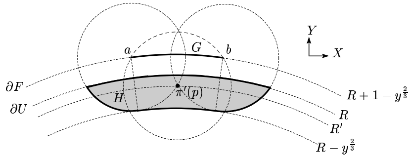
Figure 14. Section of H by a plane \Pi intersecting segment p_i p_l at p .
