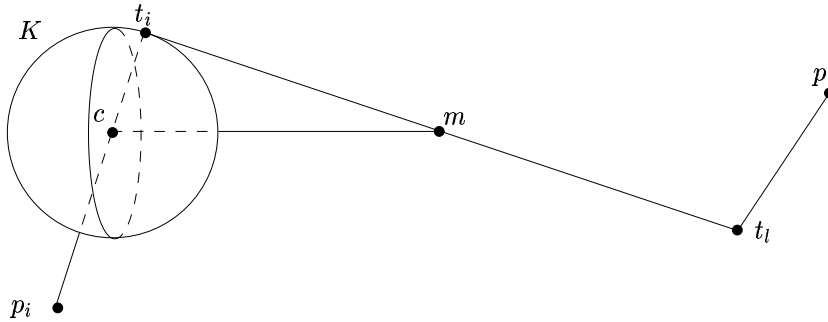
Figure 6. For the proof of Lemma 28.
