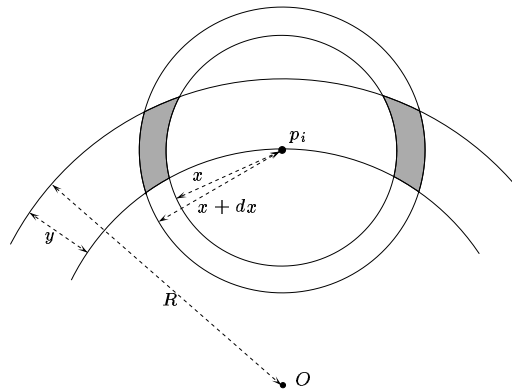
Figure 4. For the proof of Lemma 19.
