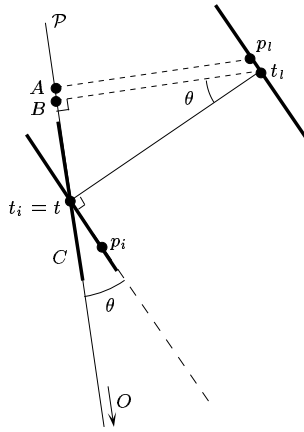
Figure 10. The height from p_l to \mathcal{P} is greater than |t_i t_l| \cos \theta - 1 .
