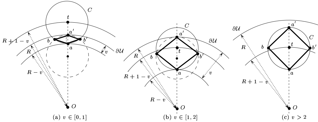
Figure 8. For the definition of t and C ( C is shown from the side view).
