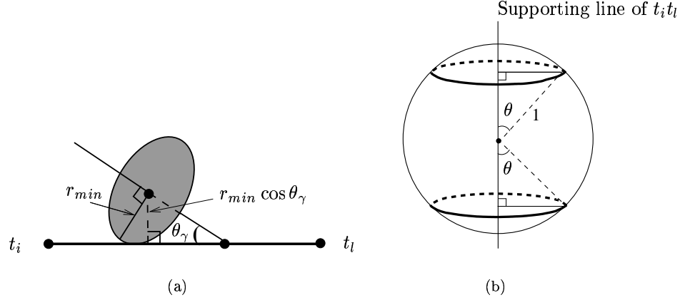
Figure 7. Illustration for the case of polygons of bounded aspect ratio.
