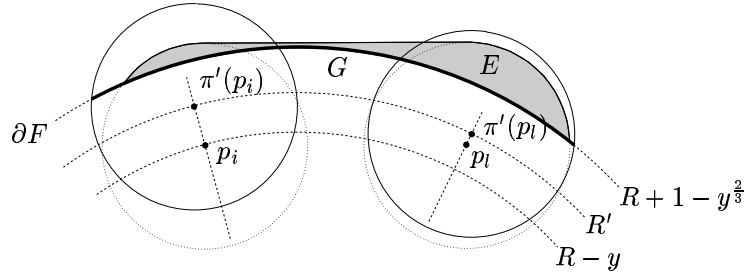
Figure 12. G , a part of \partial F enclosing E \cap \partial F .
