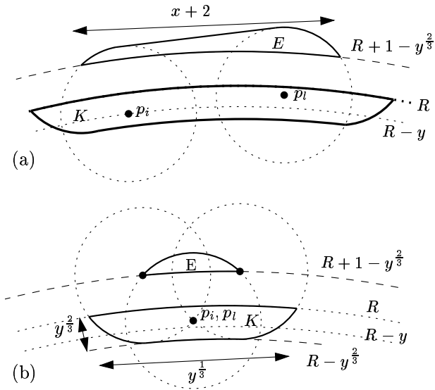
Figure 3. For the sketch of the proof of Lemma 17.
