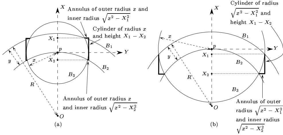
Figure 18. For the proof of Proposition 37, case 1.
