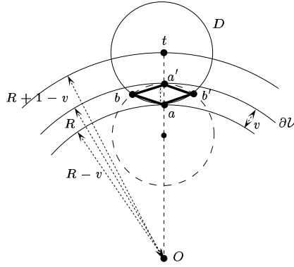
Figure 2. For the sketch of the proof of Lemma 14 ( v \in (0, 1) ).
