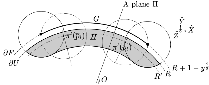
Figure 13. The region H and a plane \Pi .
