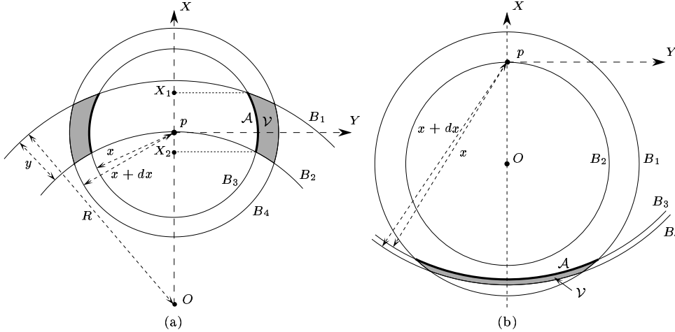
Figure 17. For the proof of Proposition 37.
