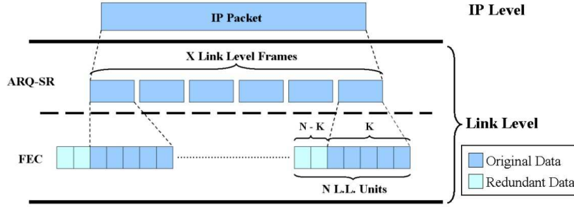
Figure 1: The Hybrid Model FEC / ARQ-SR
