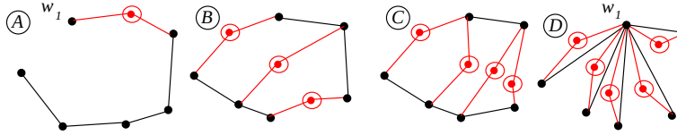
Fig. 12. \text{card}(V_0) = 6 and \text{card}(L) = 8 . The black edges represent G(L, V_0, E) and the insertion of vertices of V_2 are made using the red paths. A: \text{card}(Lu(V_0)) = 7 and m(w_1) \cap \{l\} = \emptyset ; B: \text{card}(Lu(V_0)) = 6 , three vertices of V_0 contain l in their sets of labels and the three others contain l' in their sets of labels; C: \text{card}(Lu(V_0)) = 6 , four vertices contain l in their sets of labels the two others contain l' in their sets of label; D: \text{card}(Lu(V_0)) = 6 and m(w_1) contains \{l, l'\} .
