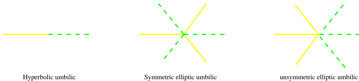
Figure 12: Ridges at umbilic
