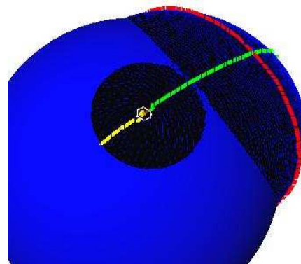
Figure 11: A_3^- contact of the blue sphere of curvature at a blue Hyperbolic ridge point (on the green curve)
