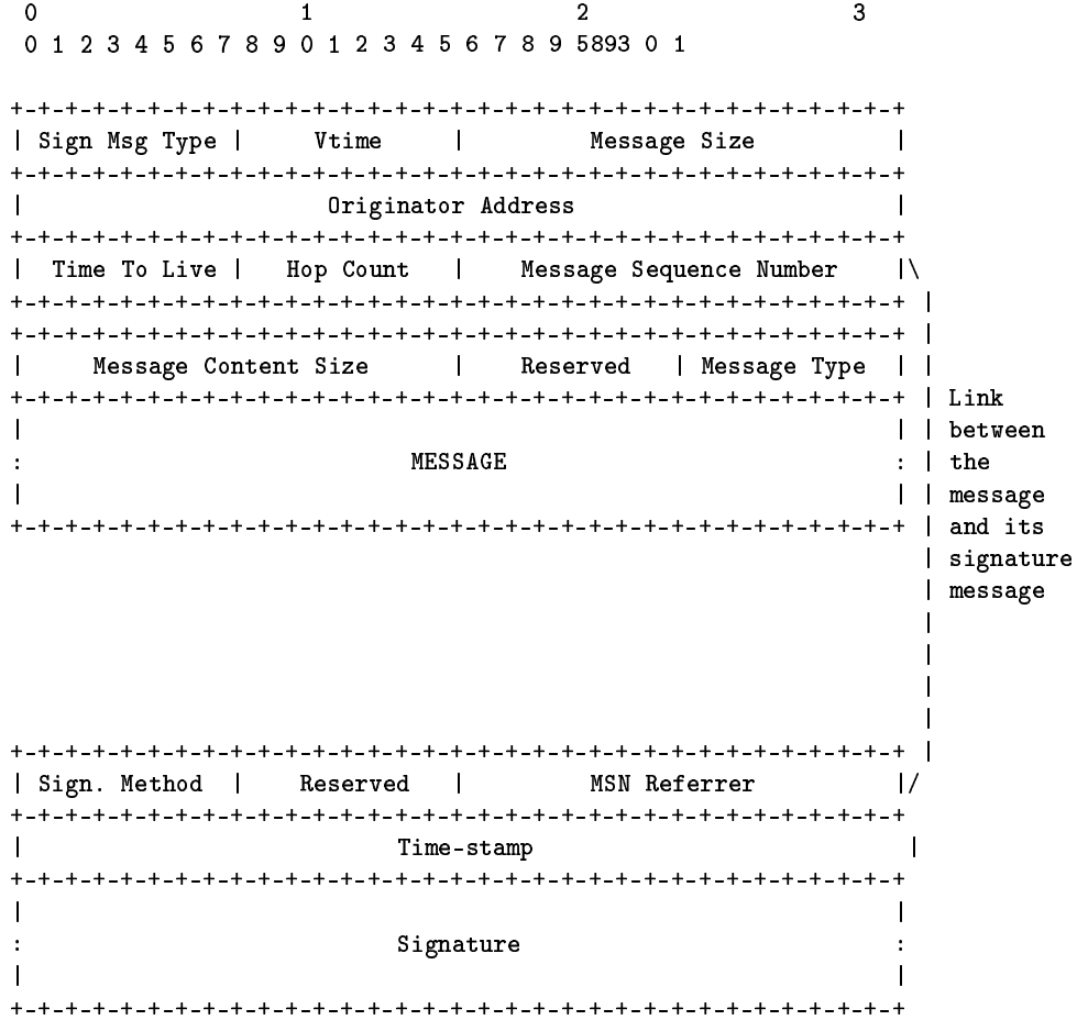
Figure 2: The controle message and its signature message.
