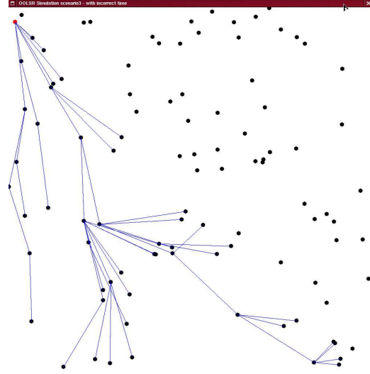
Figure 13: Routes of a node with clock offset=100
