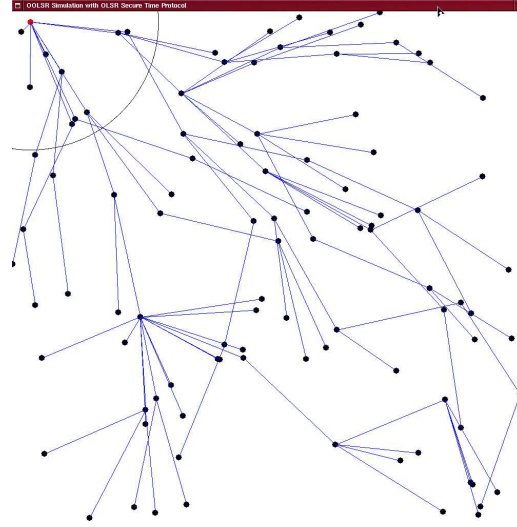
Figure 18: Simulation with OLSR Secure Time Protocol
