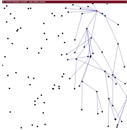
Figure 9: Routes of a node with standard messages
