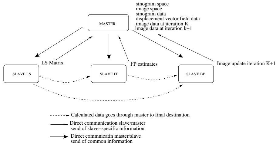
Figure 3: Implementation diagram of parallelized MLEM algorithm.
