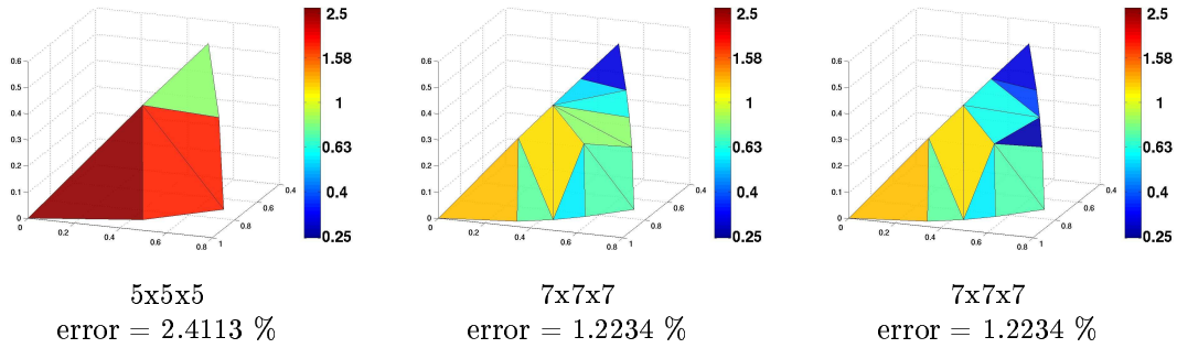
Figure 5: Errors (given in percentage) associated with the sectors of triangulated isotropic 3D chamfer masks (only 1/48 th of the sphere built from the \mathbf{n}/\|\mathbf{n}\| is depicted). From left to right, the triangulation of the 5 \times 5 \times 5 mask, the triangulation of the 7 \times 7 \times 7 mask as built in [30], and the triangulation of the 7 \times 7 \times 7 mask built by explicitly minimizing the error.
