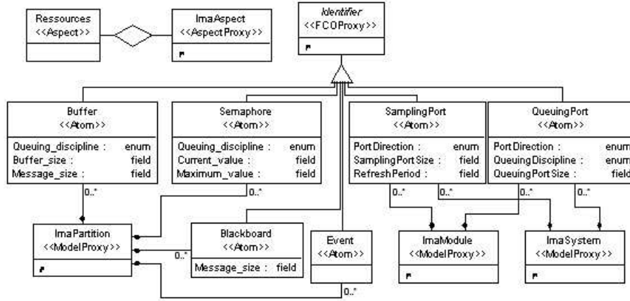
Figure 16: IMA Resource paradigm sheet.
