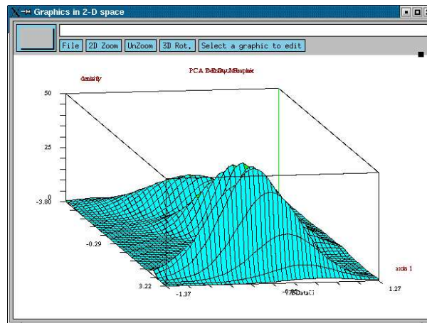
Figure 4: Density mixture in the first PCA 2D space.
