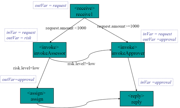
Figure 1. A loan approval process. Activities are represented in shaded boxes. The \text{inVar} and \text{outVar} are respectively the input and output variables of an activity.
