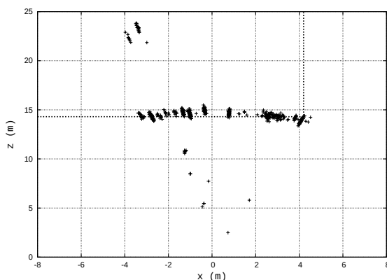
Fig. 10. Top view of flies evaluated with a fitness function using x component of Sobel gradient norms and a 23 \times 23 correlation window. The dotted lines represent the building.
