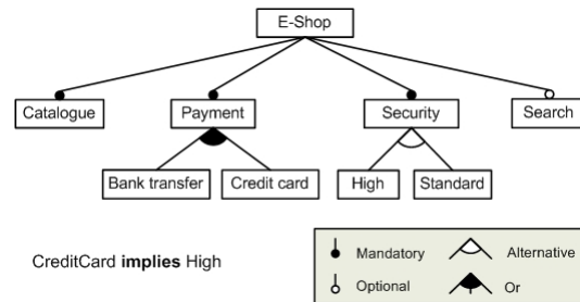
Figure 2: A Feature Model Example
