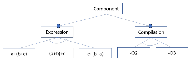
Figure 3: Simple Feature Model
