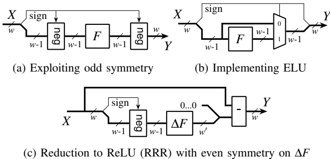
Fig. 5: Implementation techniques
