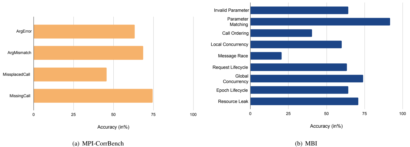
Fig. 8. Ablation study results for MPI-CorrBench (left) and MBI (right).
