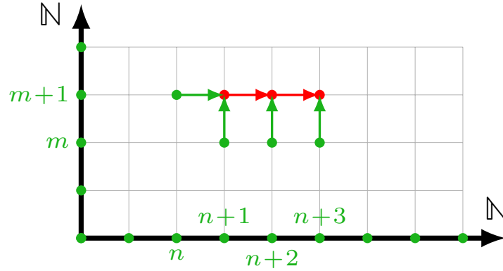
Figure 5.1: Double induction scheme “by diagonal” (see Lemma 1358).
