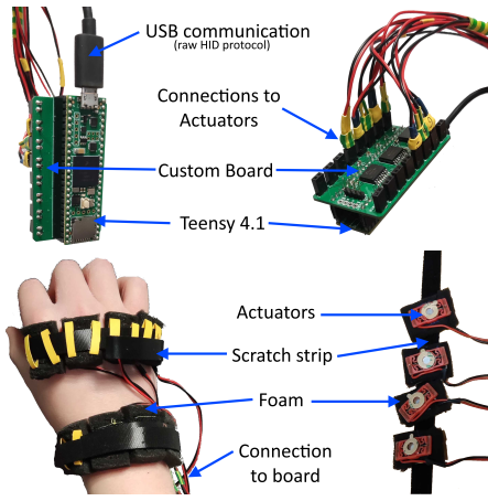
Figure 4: Apparatus used in the experiment. Left: Teesy 4.1 and custom boards. Right: actuators.
