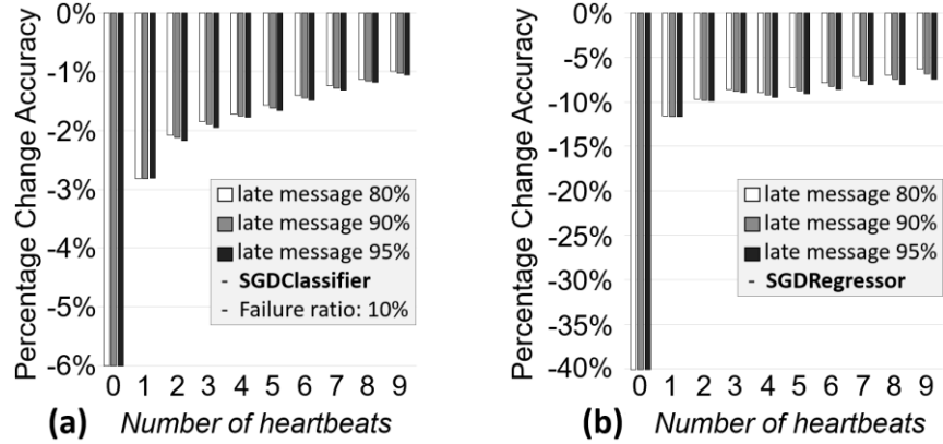
Figure 20: Heartbeat Execution Quality (SGD)
