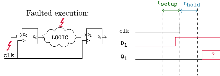
Fig. 2: Timing Fault Model on a simple circuit.
