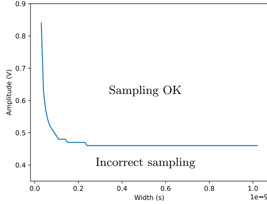
Fig. 9: Simulated sampling results: for a given glitch with voltage amplitude and width above this curve, sampling is correct.
