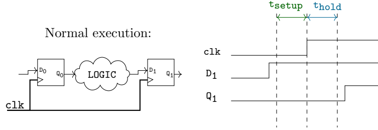
Fig. 1: Normal execution of a simple synchronous circuit.
