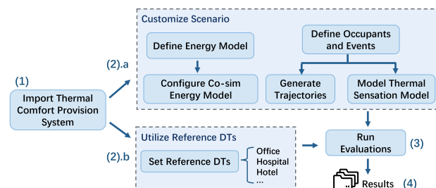
Fig. 2: Co-zyBench workflow.
