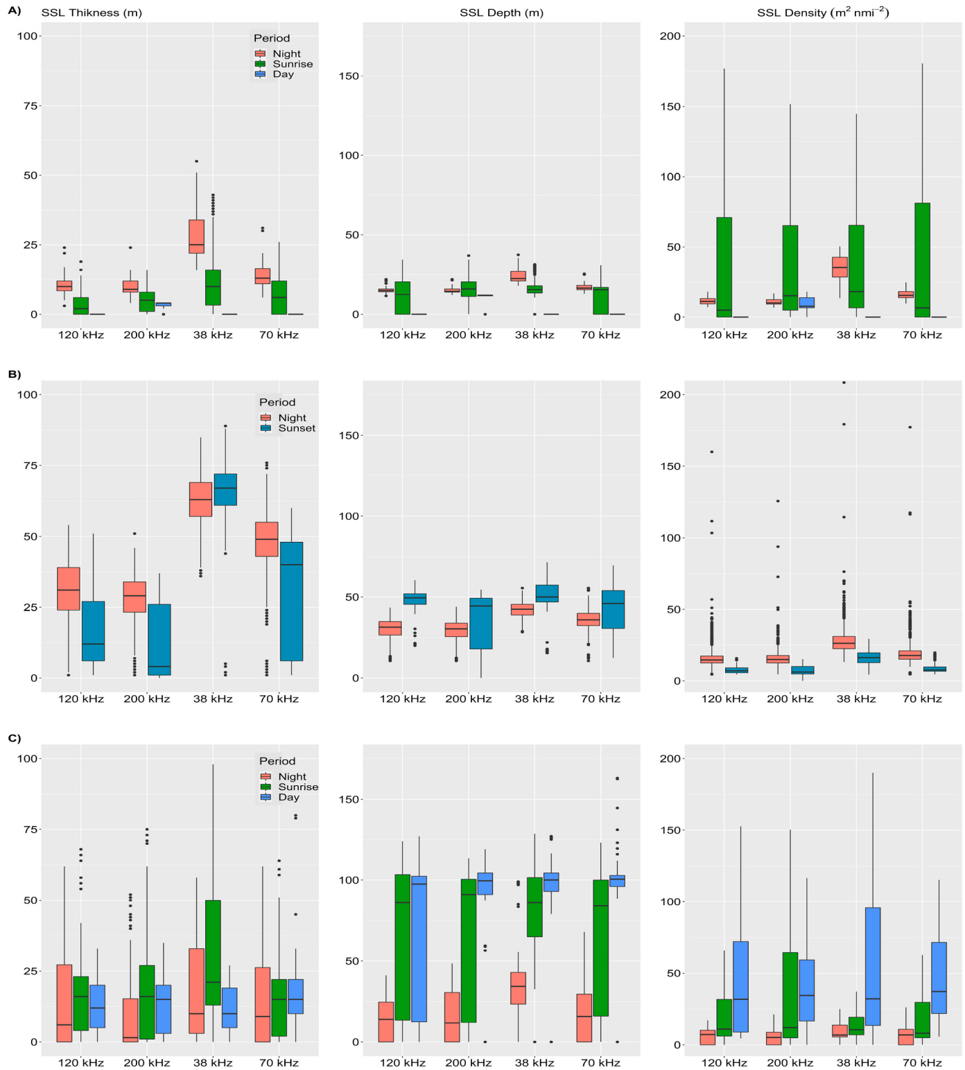
Fig. 4. Boxplot (minimum, maximum, and median) of sound scattering layer (SSL) descriptors (SSL thickness (m), SSL density (expressed in \text{m}^2 \text{nmi}^{-2} ), and SSL depth (m)) grouped by diel period (Night, Sunrise, Day and Sunset) over Senegalese waters (A: southern continental shelf; B: southern high sea and C: northern continental shelf) as observed by the echosounders during the AWA sea survey at four different frequencies (kHz).
