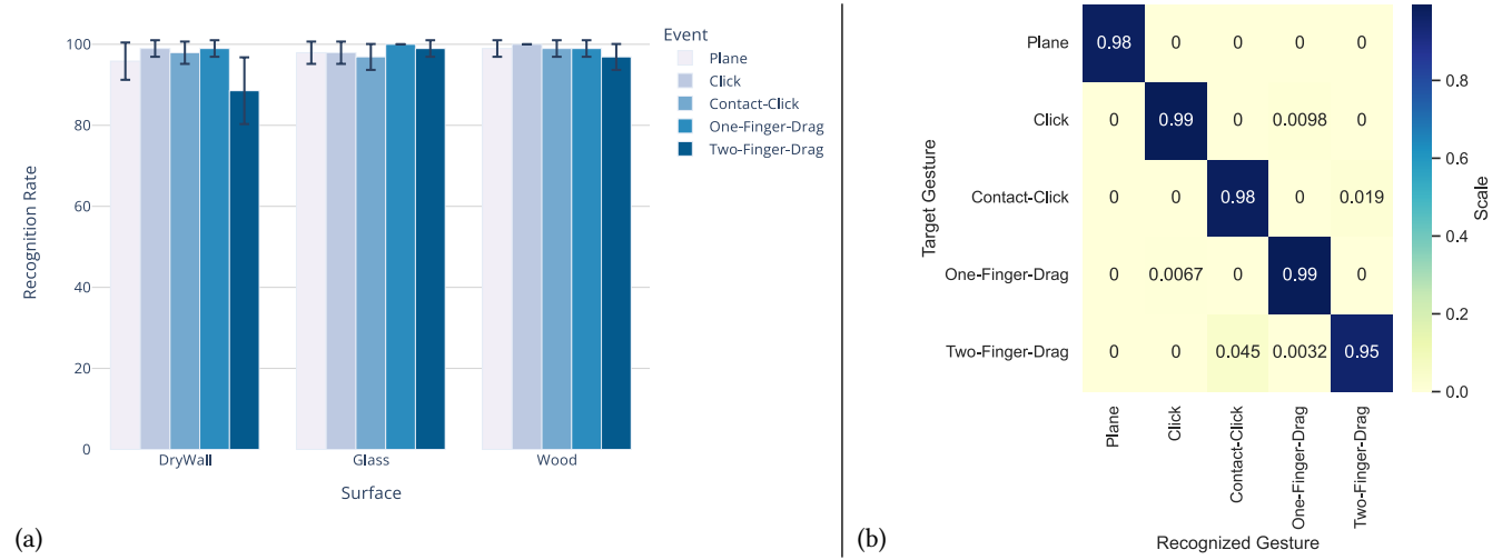
Figure 7: a) Recognition rate per SURFACE and EVENT: percentage of trials where the first event recognized by the system matched the task stimulus. Error bars represent the 95% confidence interval relative to all the data points collected in the corresponding condition. b) Confusion matrix between target gestures and recognized gestures.
