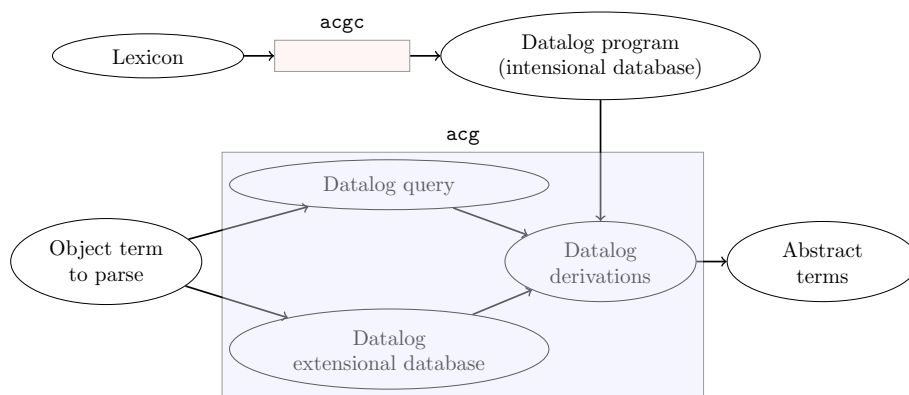
Fig. 3: Parsing process
