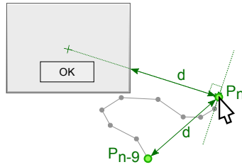
Fig. 4. AWAY displays the new GUI element so that its center is on the line perpendicular to the latest cursor displacement, and the distance between its closest edge and the last cursor location P_n is the same as between the last and 10 th last cursor location P_{n-9} .
